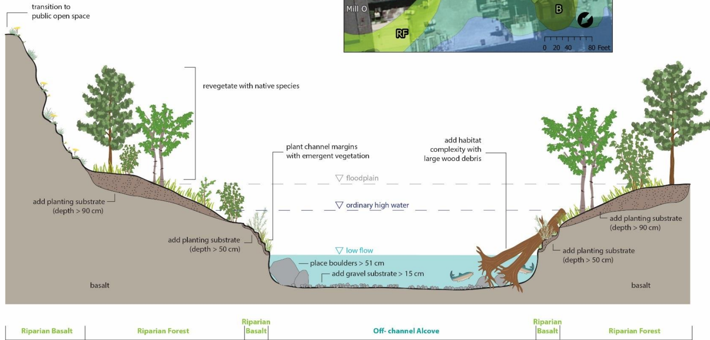
Willamette Falls Riverwalk: Habitat Design Elements Typical Alcove Detail – Plan View and Cross Section
